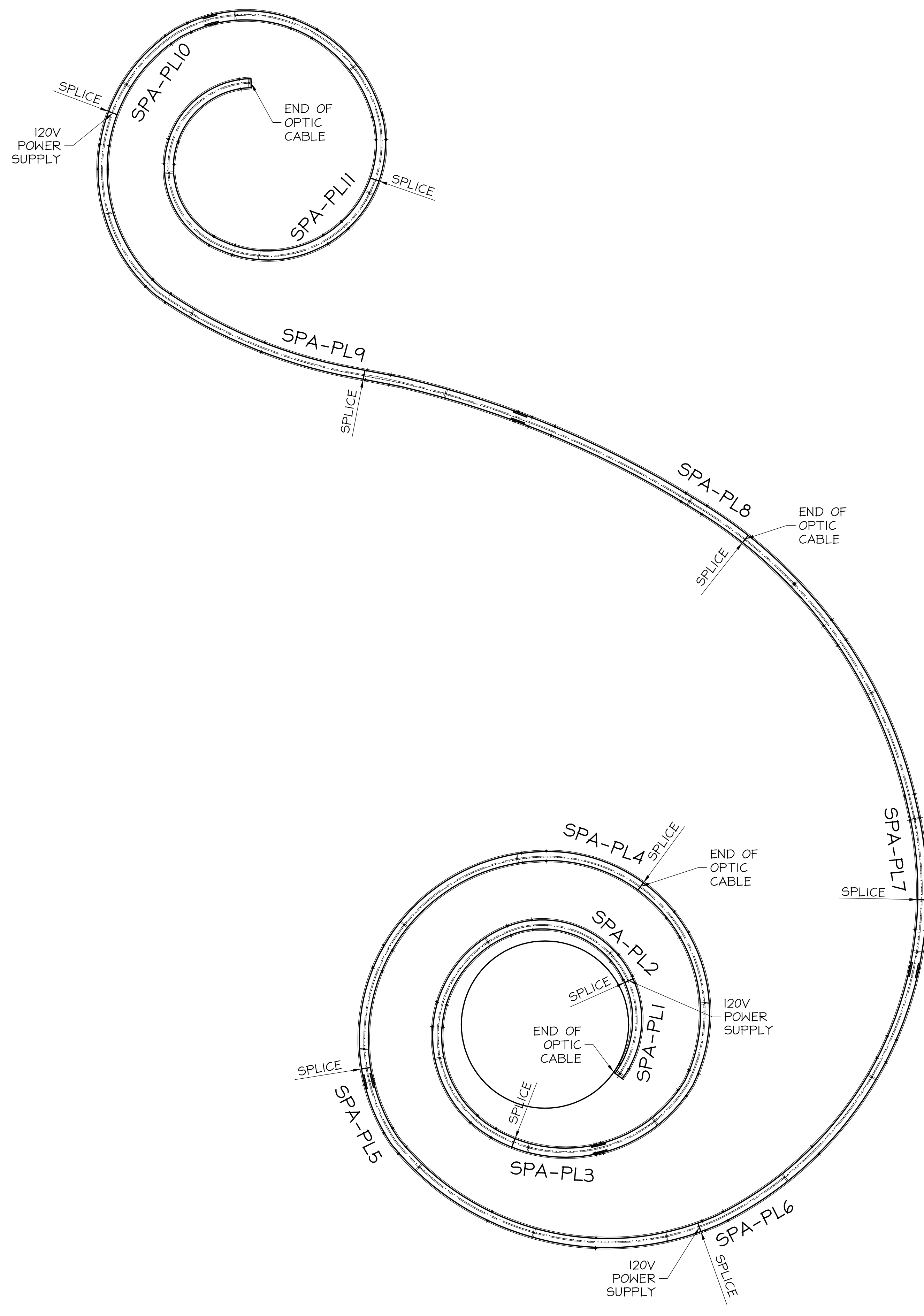
SPIRAL A PLASTIC DISTRIBUTION BAR PLAN
